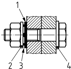
Figure 3 - Under Nut Fitting
